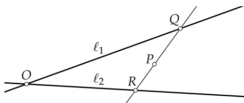
Figure 1. The reversion map.
